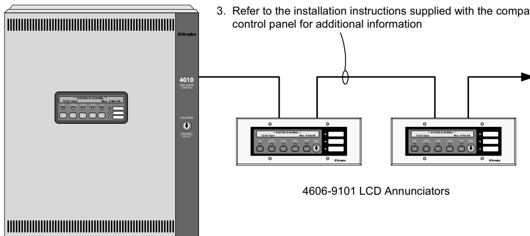
4010/4006/4008 Fire Alarm Control Panel (4010 shown for reference)
